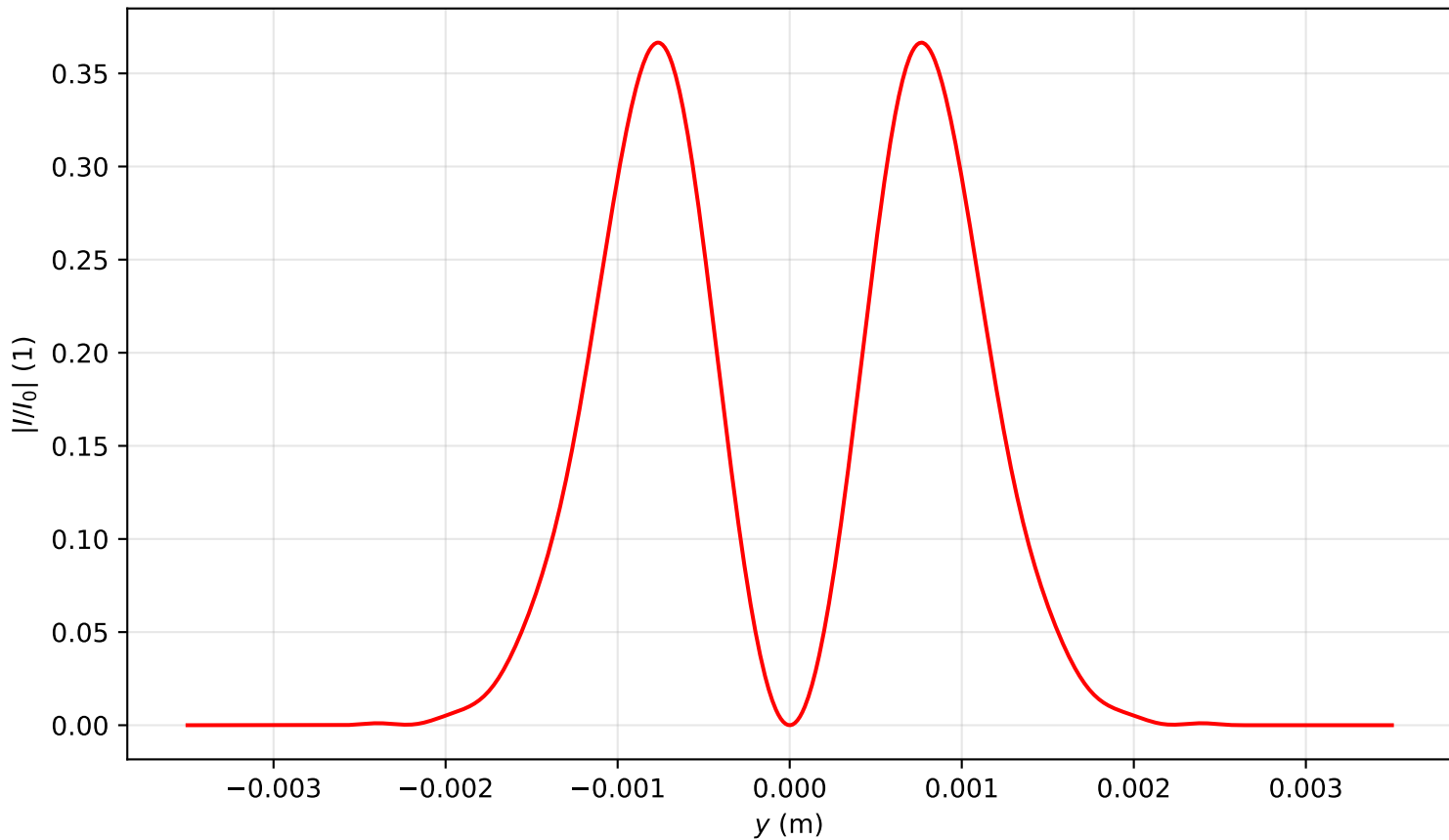
Intensity profile I(x=0, y, z=2.707)/I_0 , P_{in}=2.0P_{cr} , artificial time
